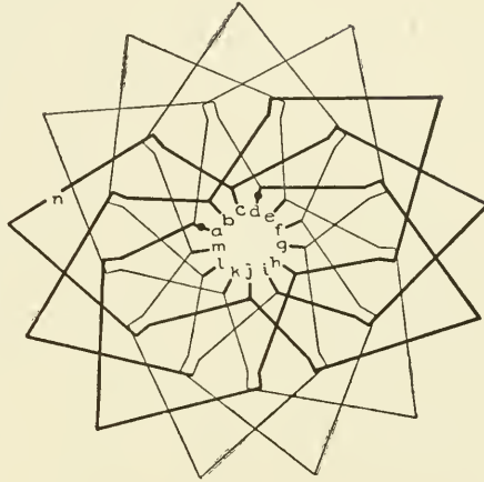
Fig. 136. Diagram Showing the Effect of an Open-Circuit in Armature Winding
